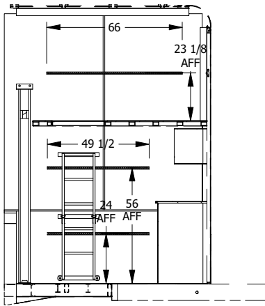
SECTION B-B SCALE 1/65
